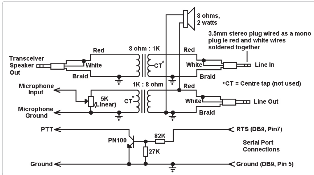
Figure 4: Schematic diagram of the 'Dibble'.
